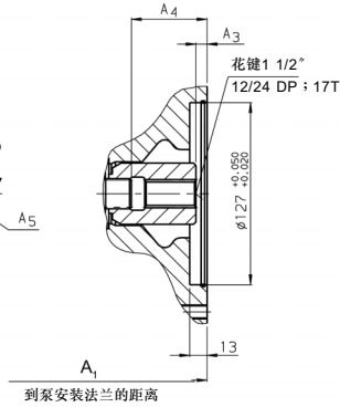
Section A - B
